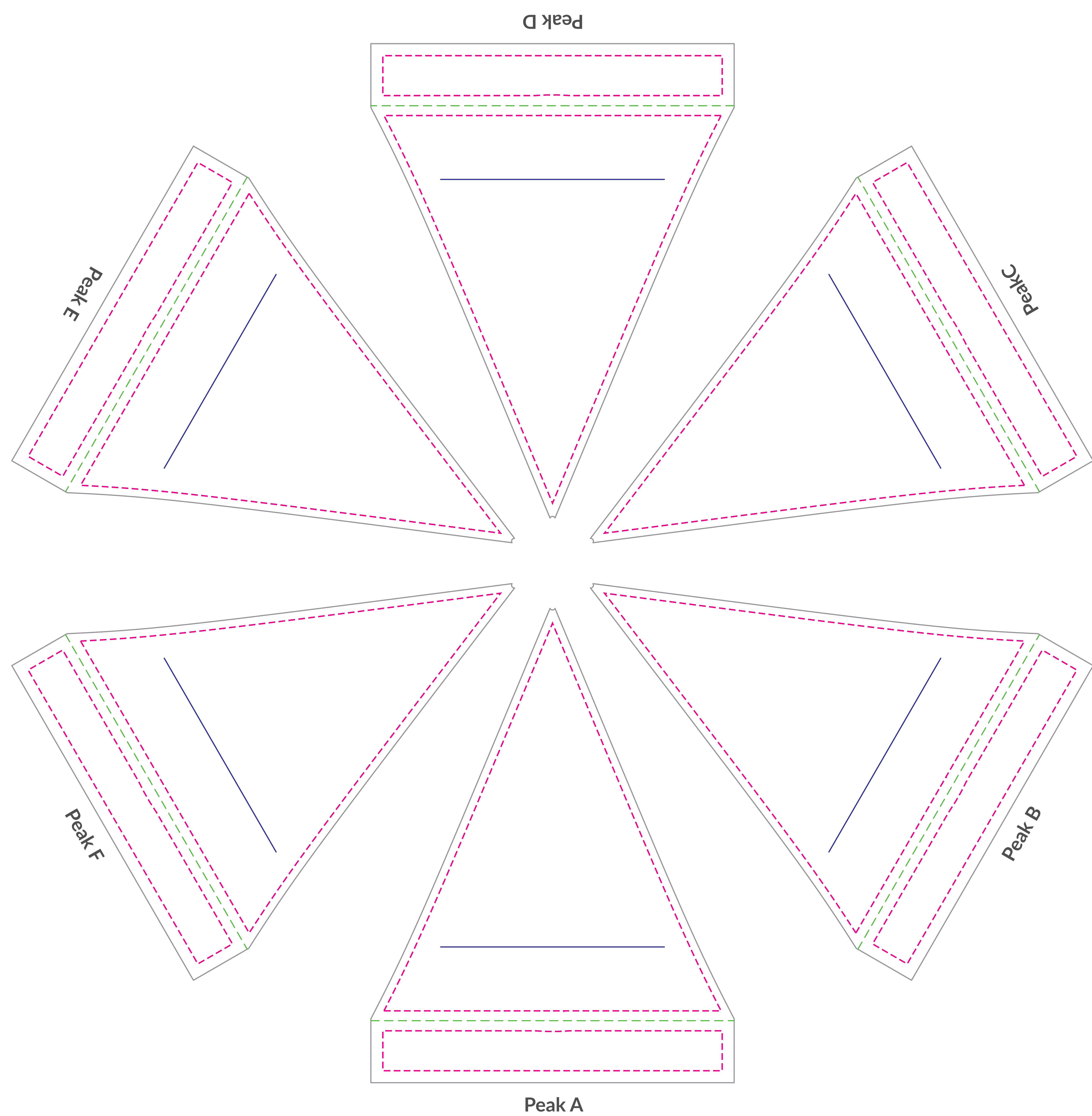
13'x15' MONARCH HEX ROOF VISUAL: 118.8”h x 91”w PEAK SAFETY: 97.2”h x 84.4”w VALANCE SAFETY: 10”h x 85”w
